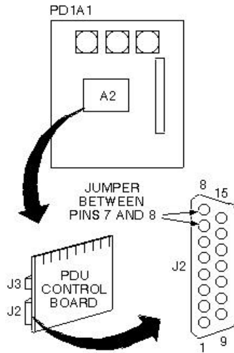
ILLUSTRATION L2697A EMERGENCY STOP JUMPER
